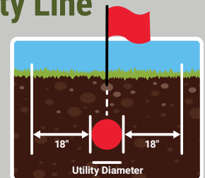
Tolerance Zone
